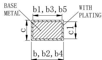
SECTION C-C, D-D&E-E
