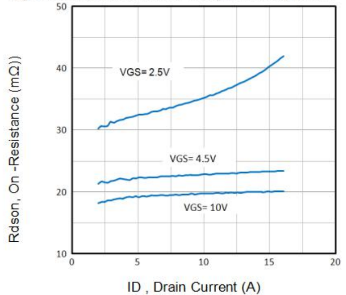
Fig4. On-Resistance vs. Drain Current and VGS
