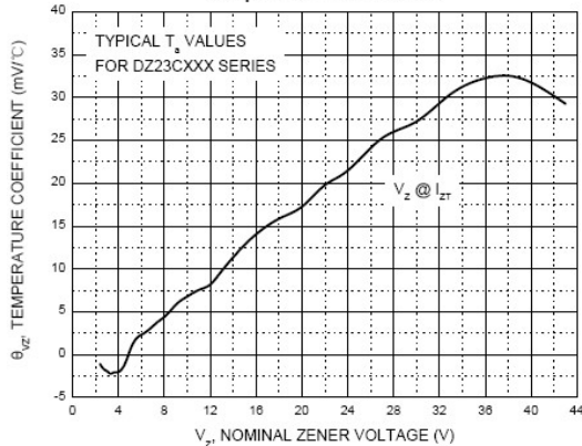
Temperature Coefficients
